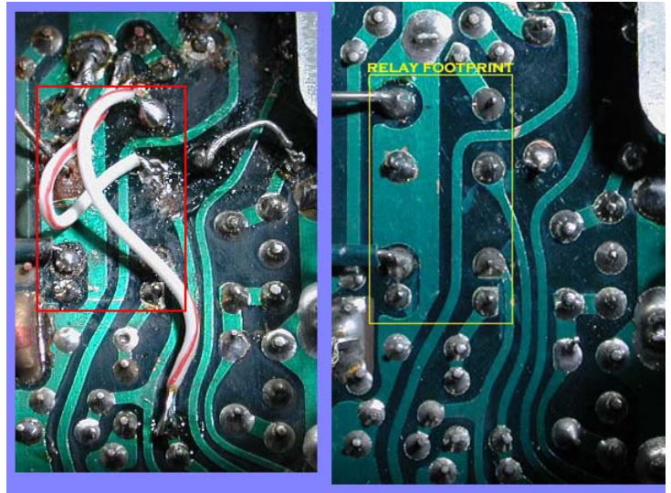
Modified board
