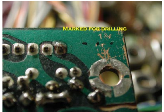
Figure 5 - Using the 7808 pins as a template (or calipers, ruler of some other measuring tool) mark the board and then drill the holes.
