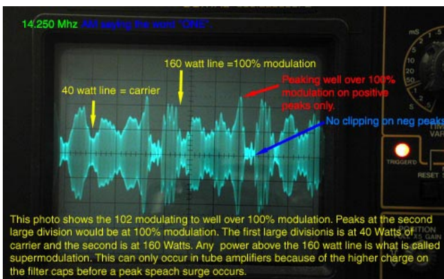
Figure 1 - Scope display of a properly tuned and operating FT-102 on AM.
